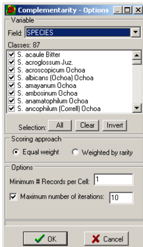
Figure 12. The Complementarity options window
