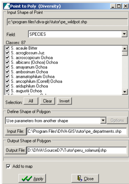
Figure 13. Point to polygon window
